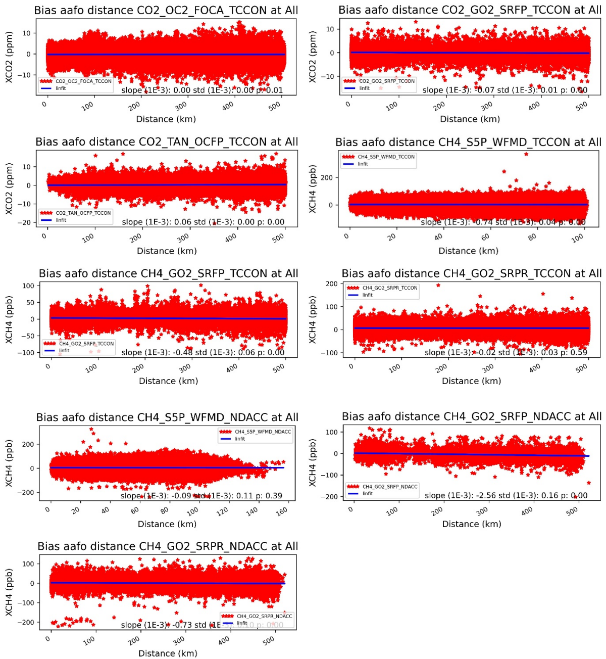
Figure 4-3: Satellite-TCCON or NDACC bias as a function of (afo) distance between the satellite and TCCON/NDACC sampling point, for all algorithms in this study. Slope in ppm/100 km for XCO 2 and ppb/100 km for XCH 4 .
