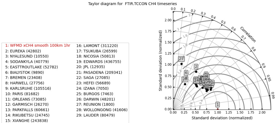
Figure 4-18: Taylor plot of daily averaged XCH 4 TCCON values relative to CH4_S5P_WFMD. Straight lines correspond with the correlation, light grey lines yield the variability of the TCCON data relative to the satellite variability and the dark grey lines correspond with the variability of the Satellite -TCCON bias relative to the satellite variability.
