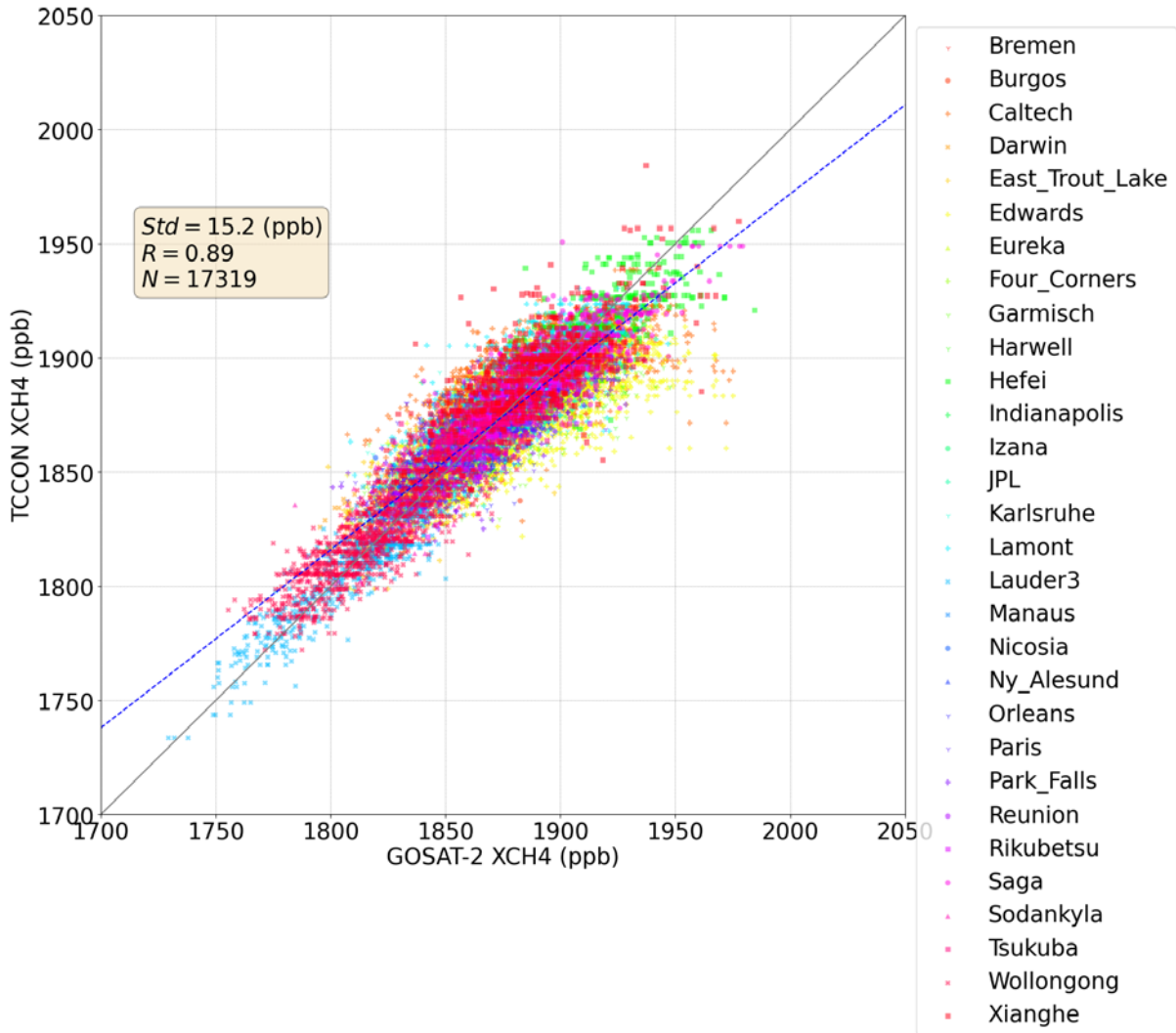
Figure 5.5-2: GOSAT-2 XCH 4 for soundings over land plotted against TCCON, for the RemoTeC Full Physics product. Data are compared only if they are fully colocated in space and time. The standard deviation of the population, Pearson's correlation coefficient and number of retrievals are given in the inset. The legend plots the different TCCON stations where markers are as follows. Stations that are along the coast and also sensitive to glint mode (ocean) measurements are indicated as circles. Those that have high latitudes in the northern and southern hemispheres are upward triangles and crosses, respectively. Stations in Asia, North America and Europe are indicated by squares, pluses and downward triangles respectively.
