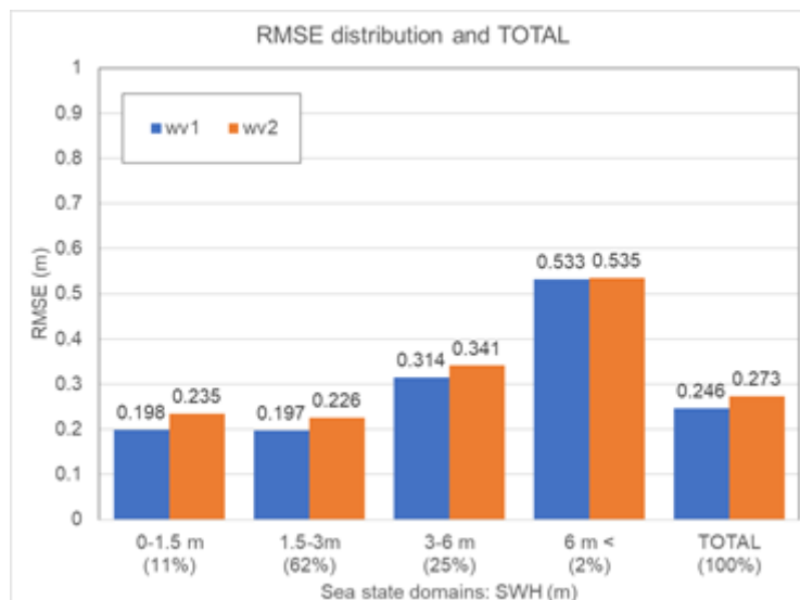
Figure 5.2. Distribution of RMSE_{CMEMS} for different sea state domains.
