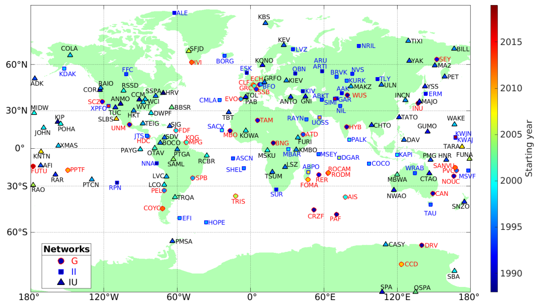
Figure 1: world map showing locations of the seismic stations from the Geoscope (G), IRIS-IDA (II) and IRIS-USGS (IU) networks and for which data is provided, starting in the year indicated by the color code.
