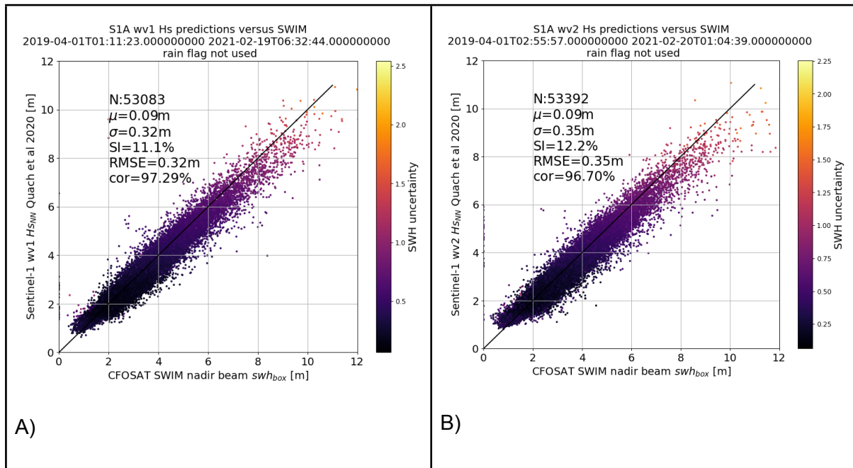
Figure 5.1 A) and B) are examples of SWH performances for WV1 (resp. WV2) with respect to SWIM nadir 1Hz measurements in open ocean with acquisitions in between 55° North and 55° South (to avoid sea-ice or icebergs contaminations).
