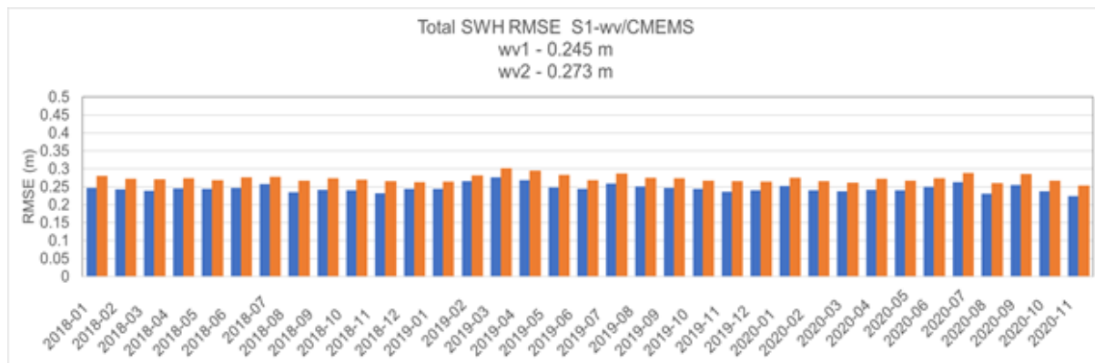
Figure 5.3. Variation of monthly estimated total RMSE_{CMEMS} for wv1 (blue) and wv2 (orange).
