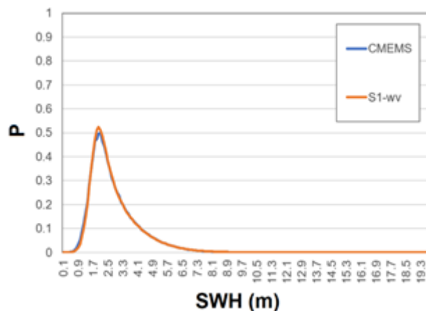
Figure 5.4. Histogram of significant wave height SWH from S1 wv and CMEMS, built using 10cm bins for whole S1 wv archive 2018-2021 including all 3.6Mio samples.
