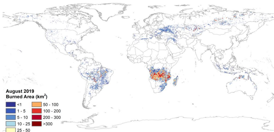
Figure 3.2: Example of the Burned Area attribute of the 20190801-ESACCI-L4_FIRE-BA-MODIS-fv5.1.nc file.
